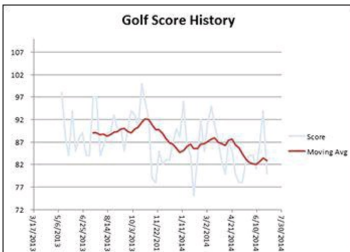
Figure 8-5: The moving average is charted over the raw scores.
