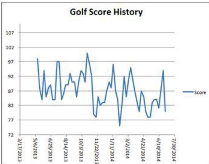
Figure 8-4: A graph of raw golf scores over time.
