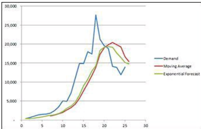
Figure 8-7: A chart comparing raw data, a simple moving average, and an exponential forecast.
